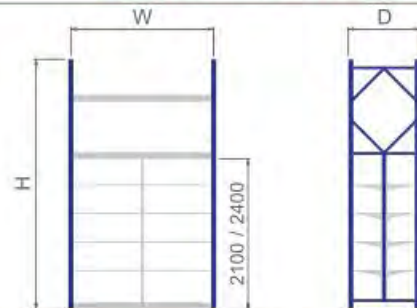
RACKING DIMENSION (mm.)
